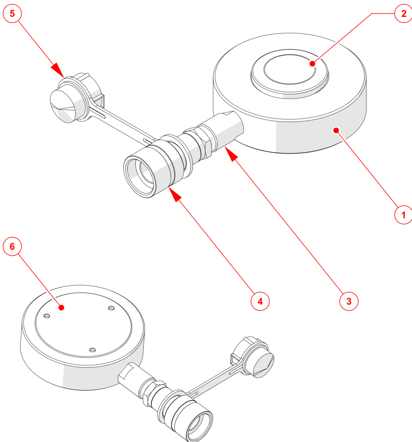
Figure 4.1: Component Identification
