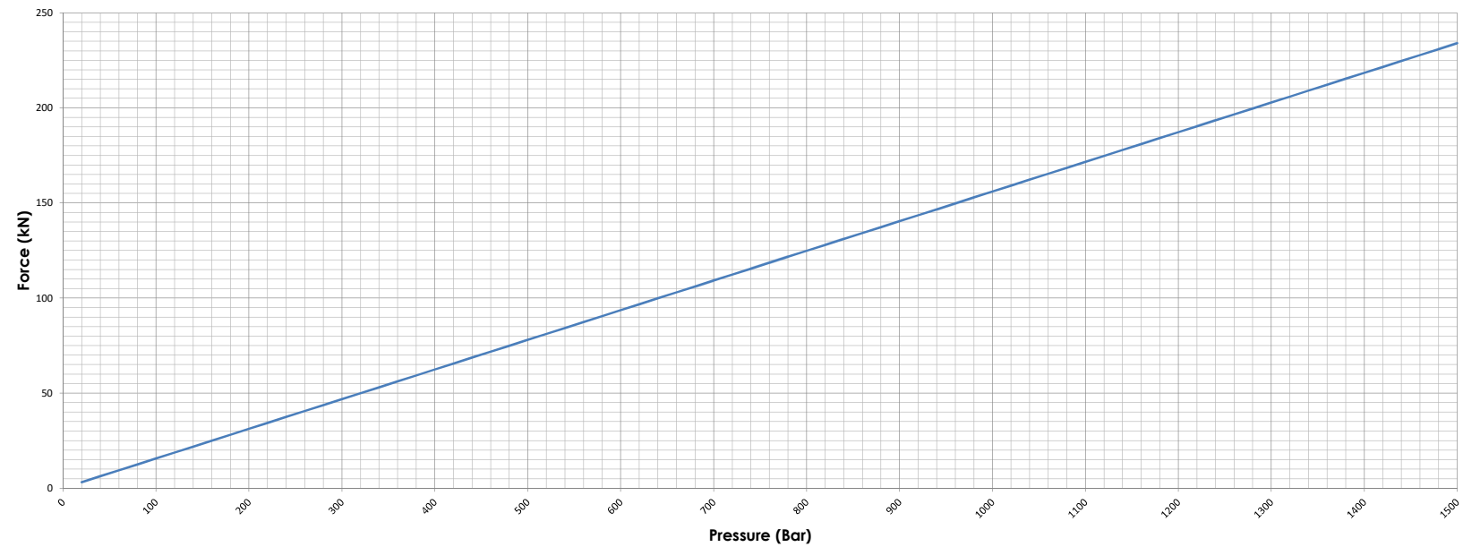
STS1 TENSIONING PRESSURE TO FORCE CONVERSION CHART (kN/Bar)
