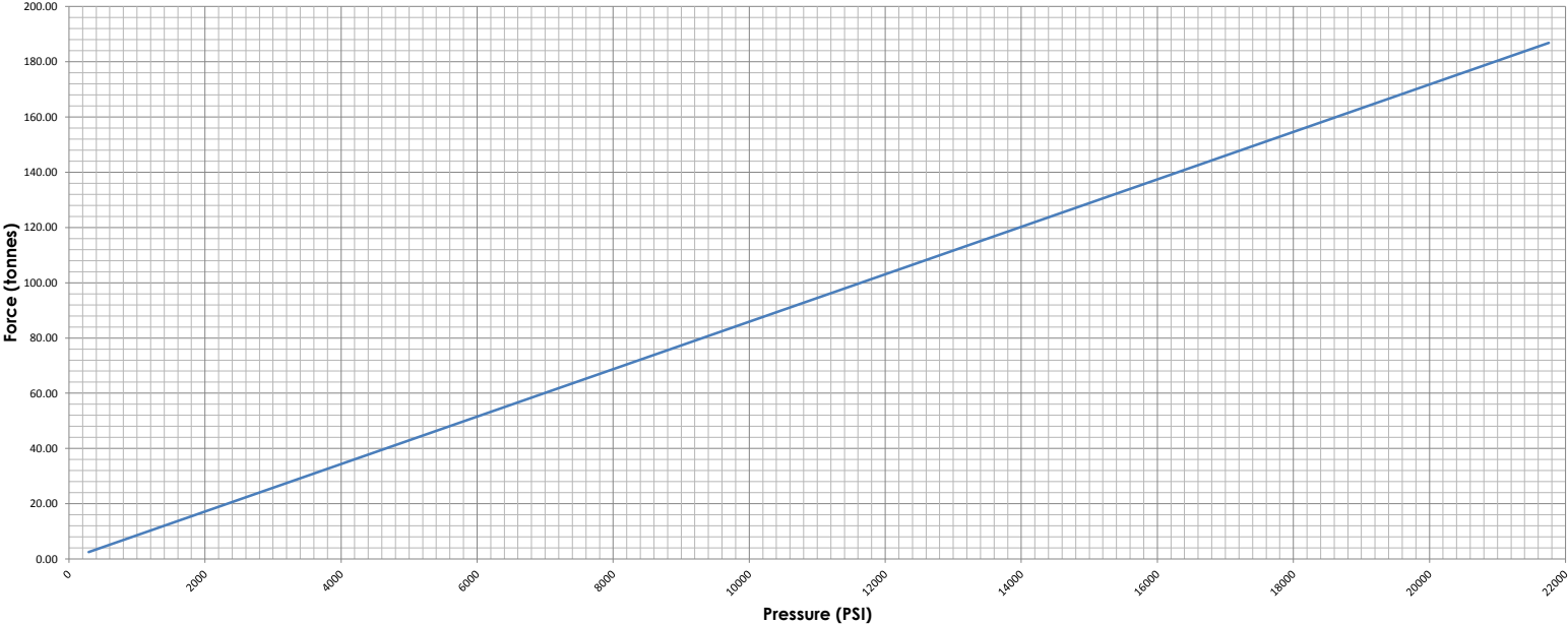
ST55 & SBT5 TENSIONING PRESSURE TO FORCE CONVERSION CHART (tonnes/PSI)
