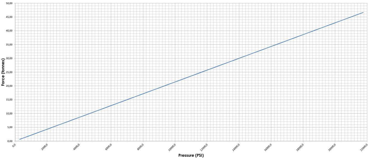
STS2 & SBT2 TENSIONING PRESSURE TO FORCE CONVERSION CHART (tonnes/PSI)
