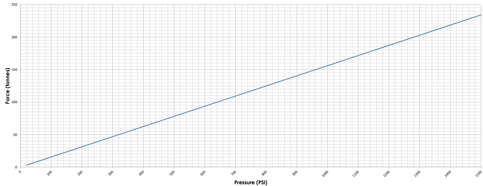
STS1 TENSIONING PRESSURE TO FORCE CONVERSION CHART (tonnes/PSI)
